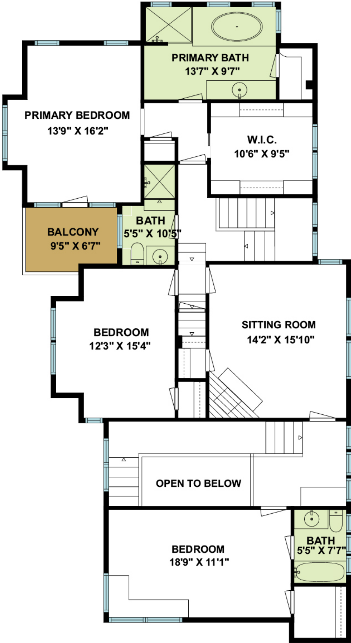
SECOND FLOOR
