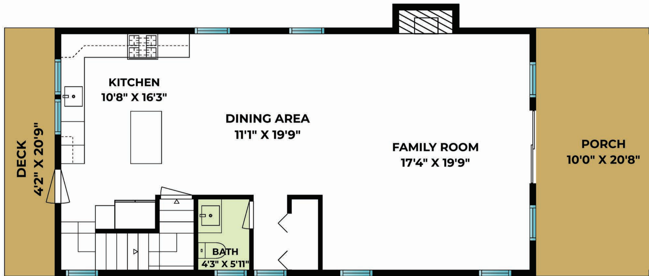
FIRST FLOOR
