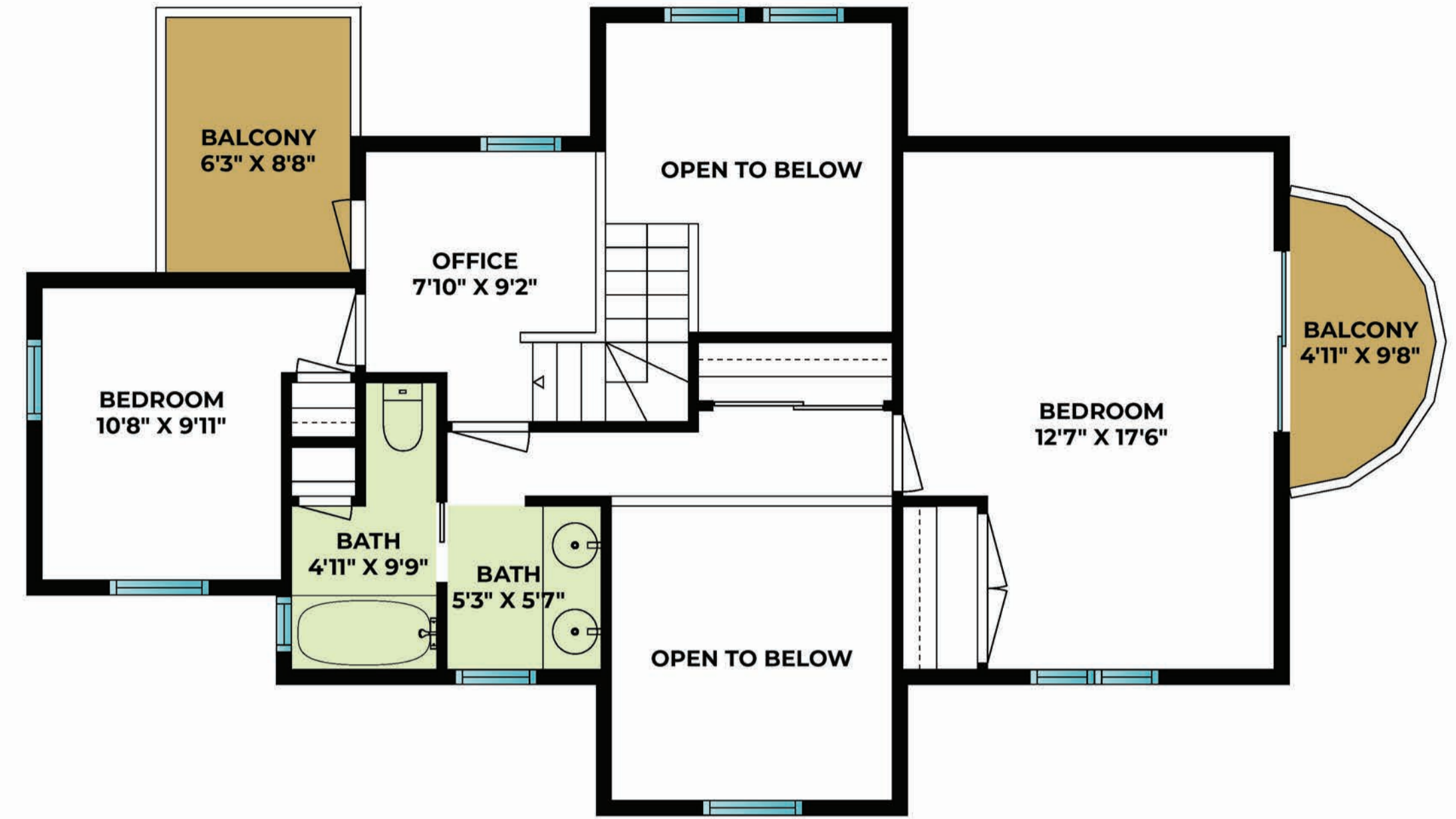
SECOND FLOOR
