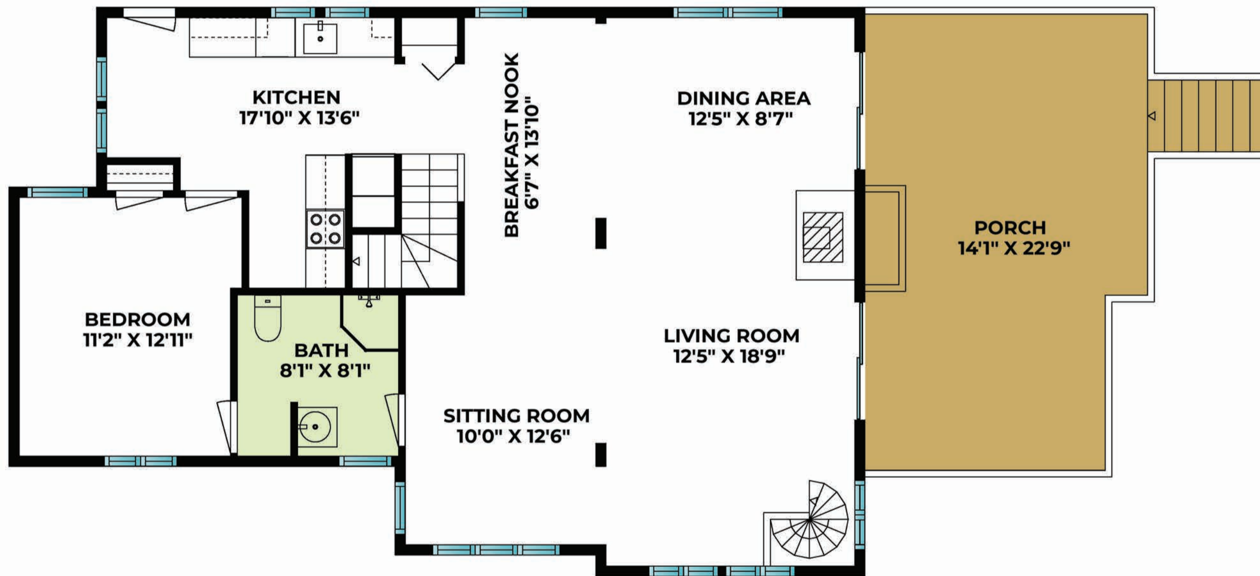
FIRST FLOOR
