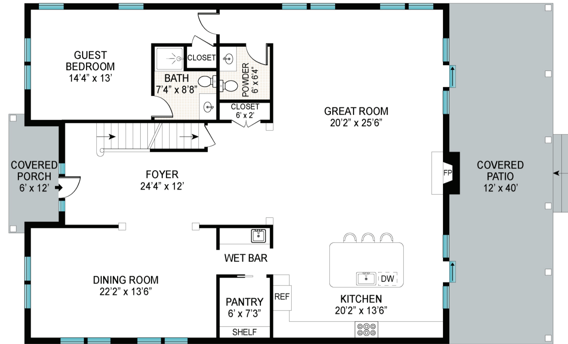
FIRST FLOOR
