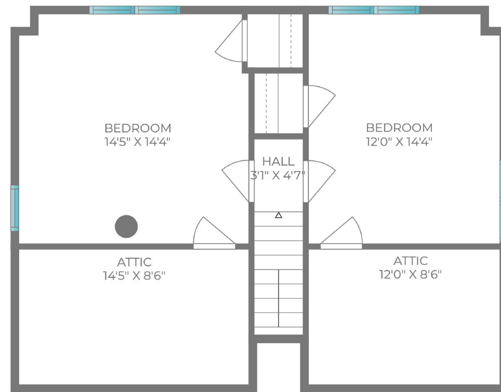
SECOND FLOOR
