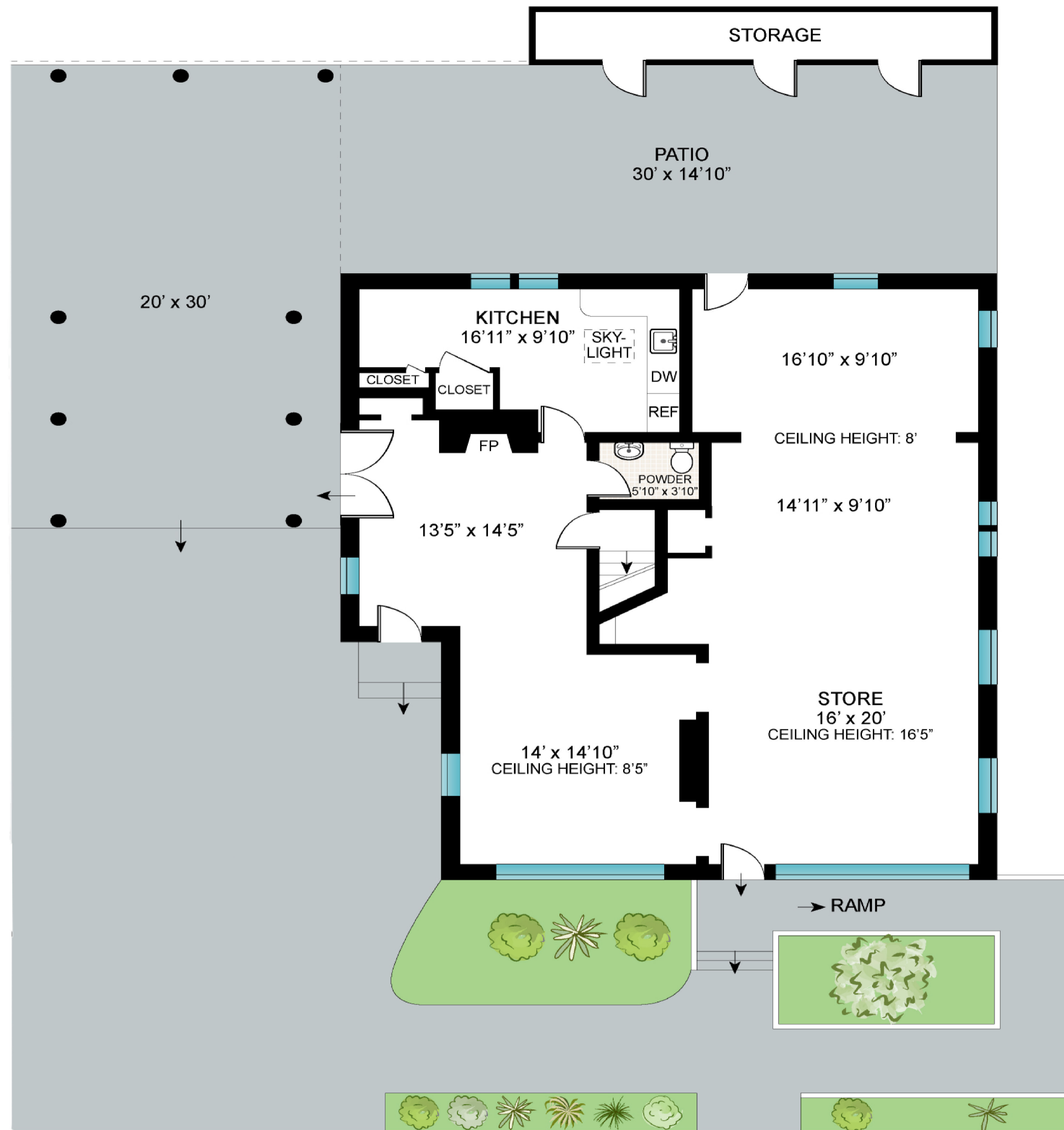
FIRST FLOOR
