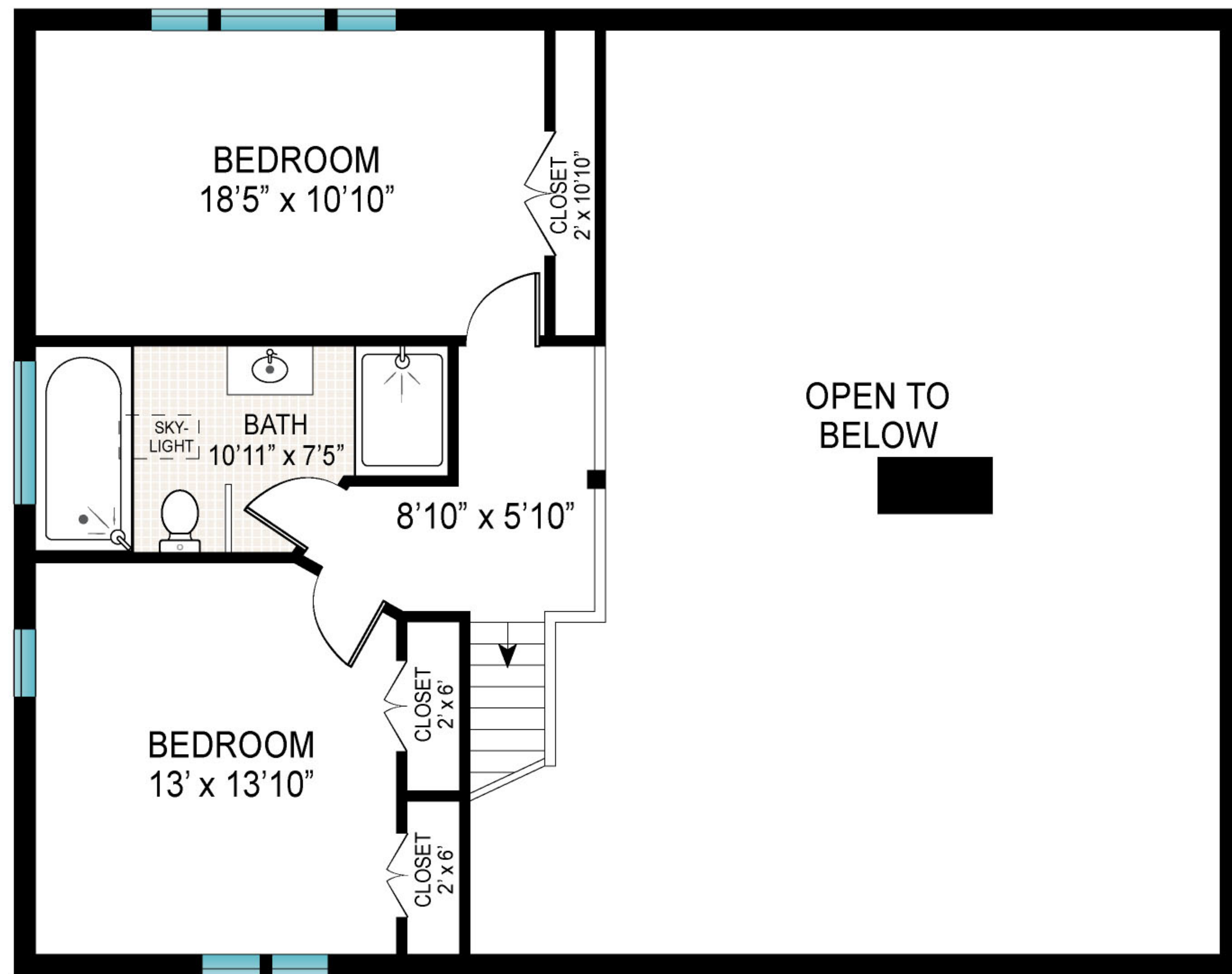
SECOND FLOOR
