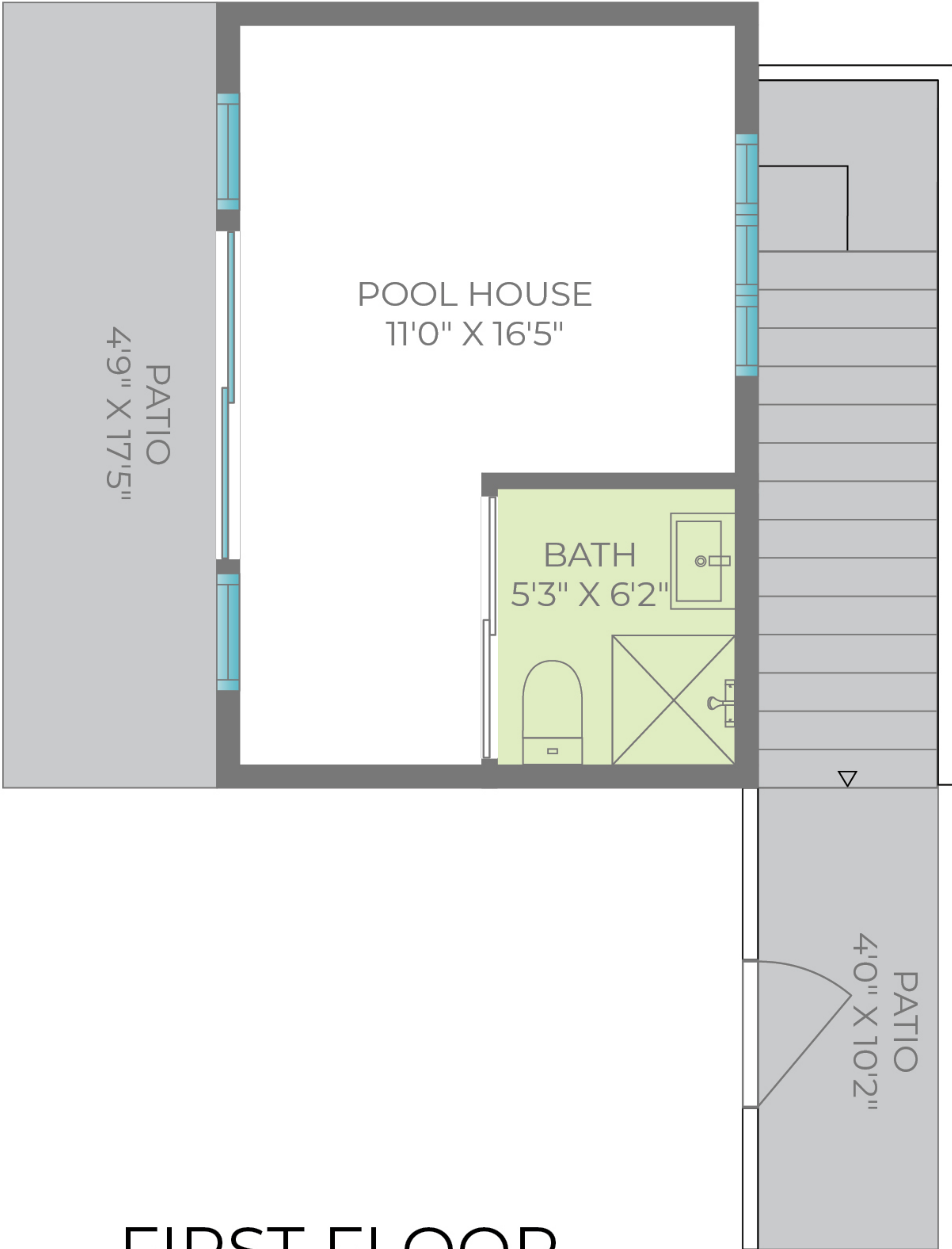
FIRST FLOOR
