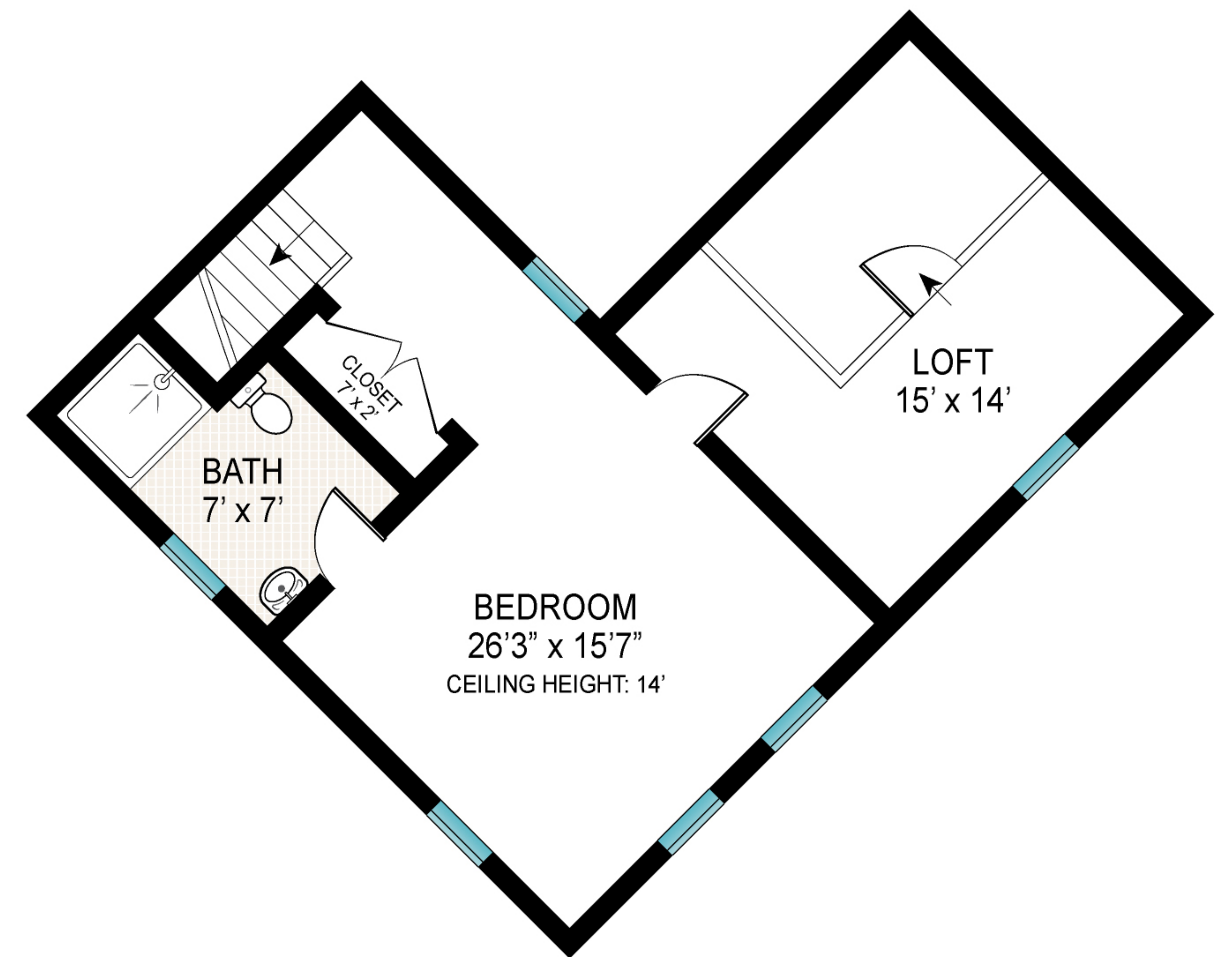
SECOND FLOOR
