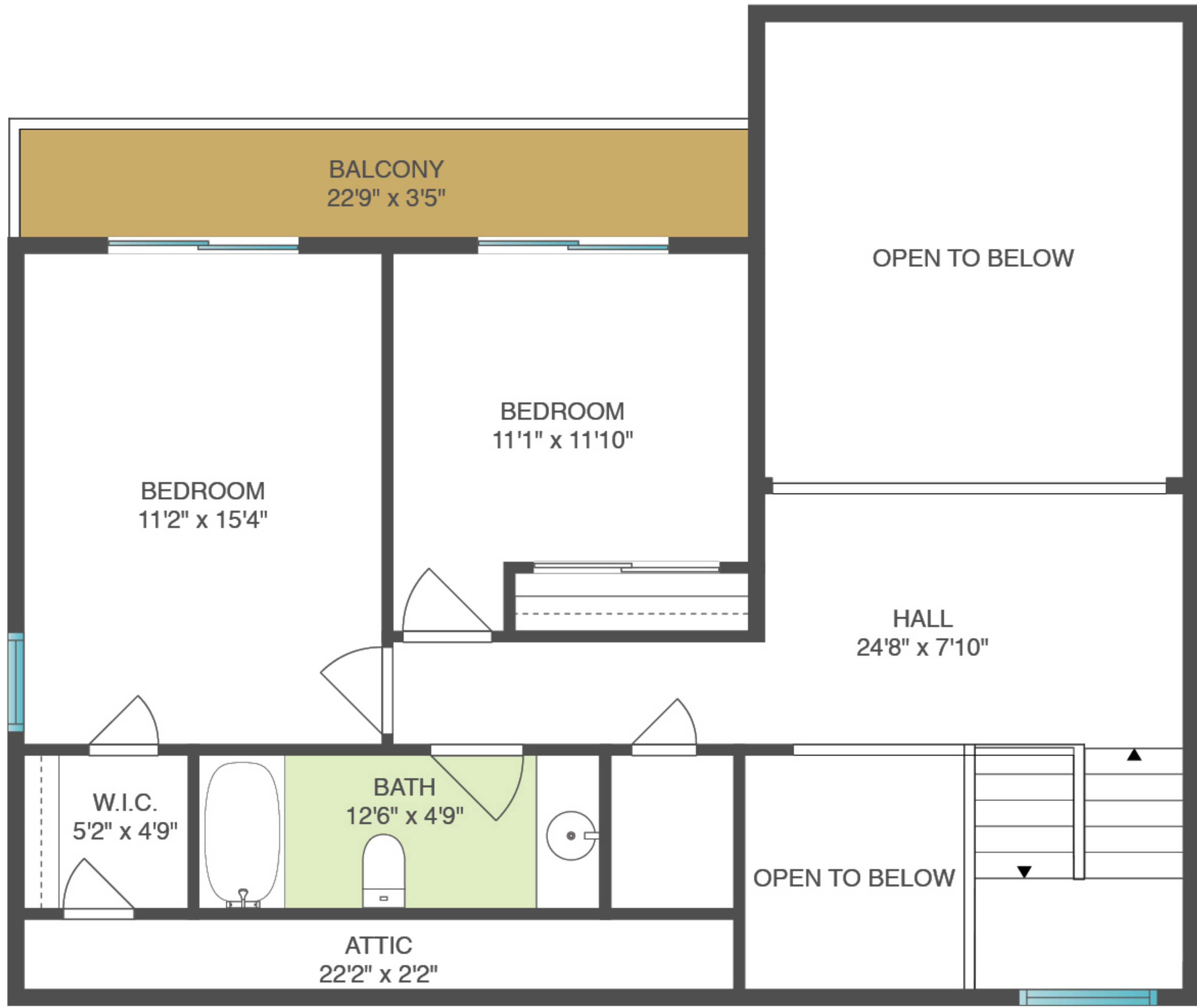
SECOND FLOOR
