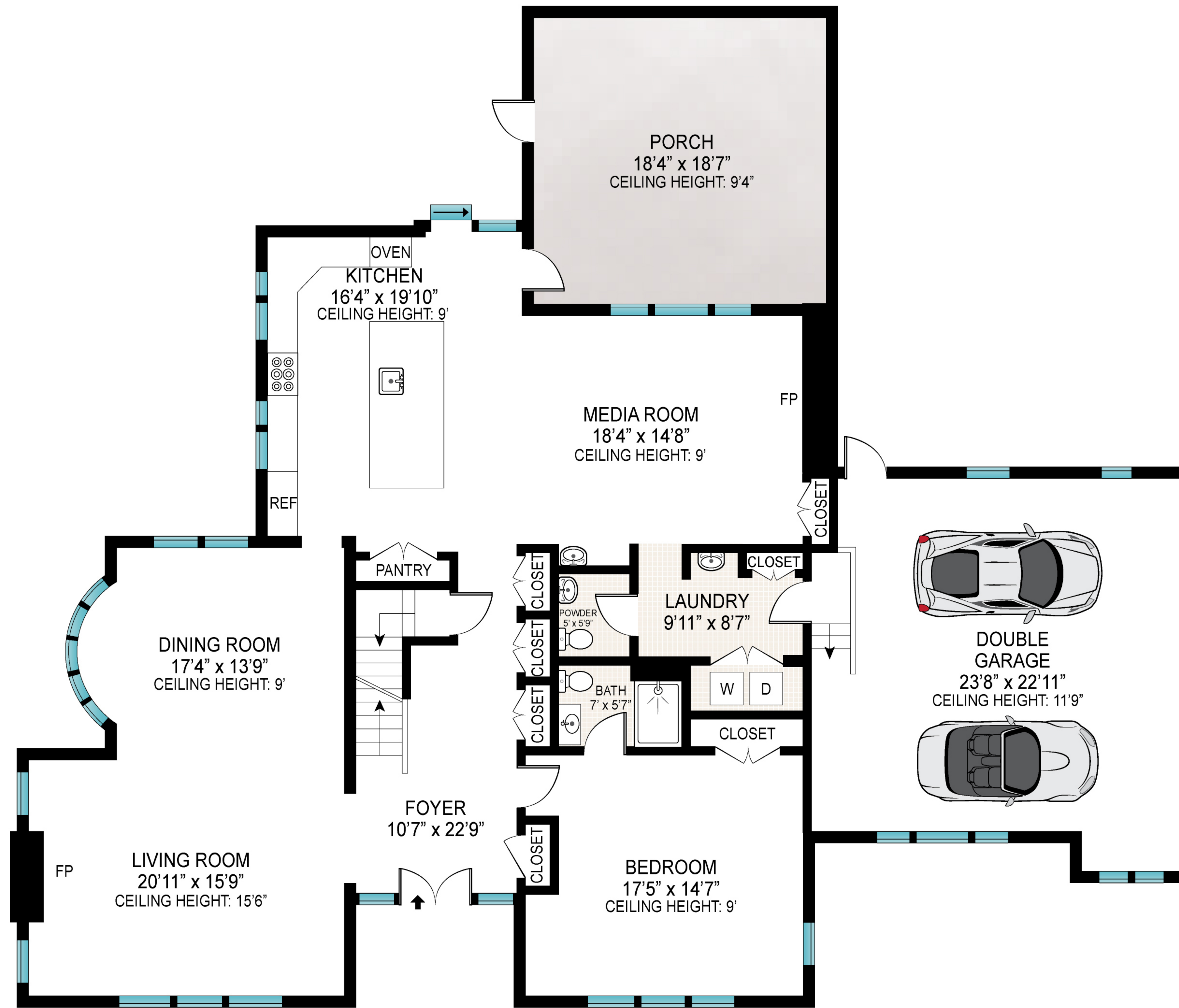
FIRST FLOOR
