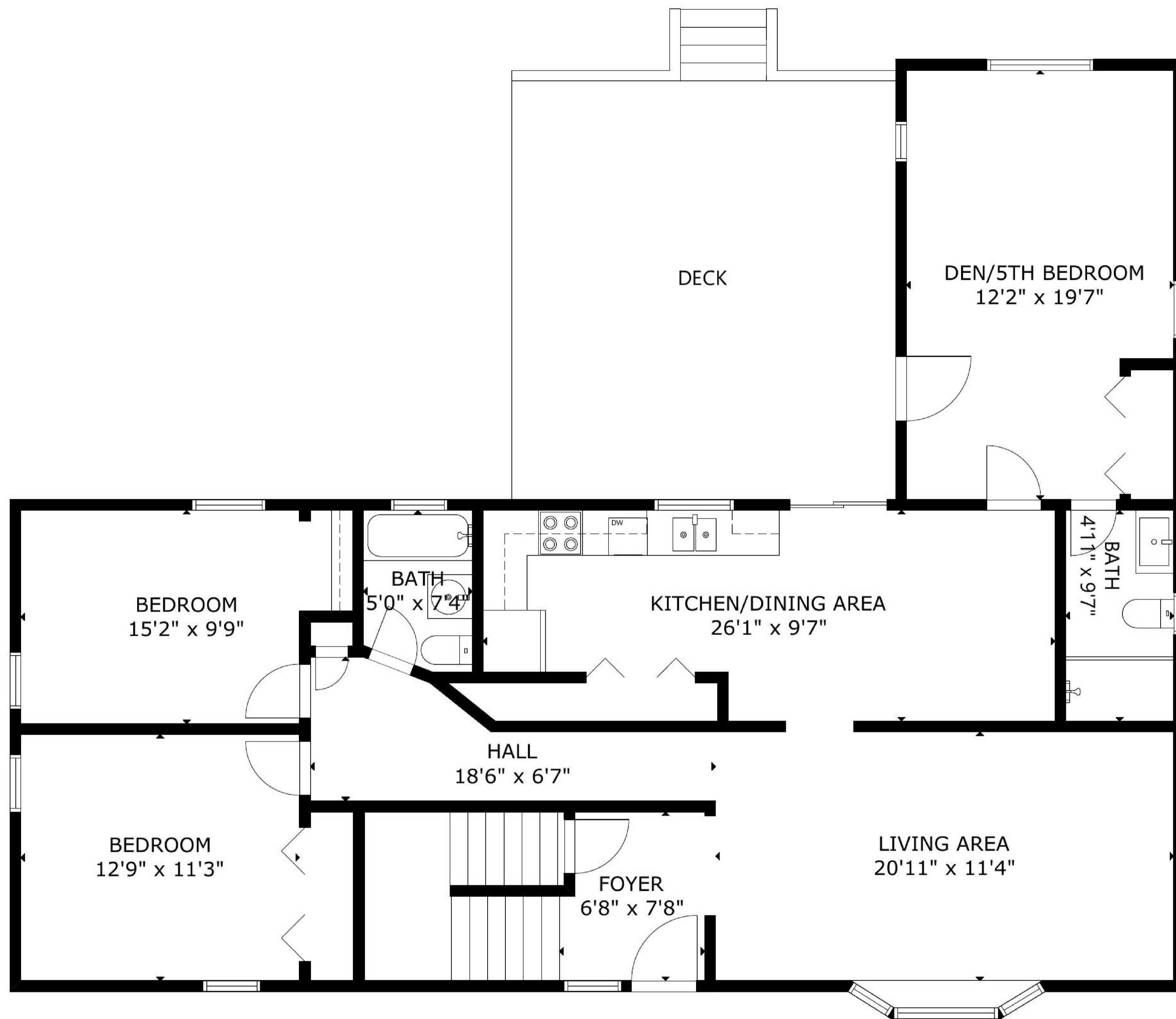
FIRST FLOOR
