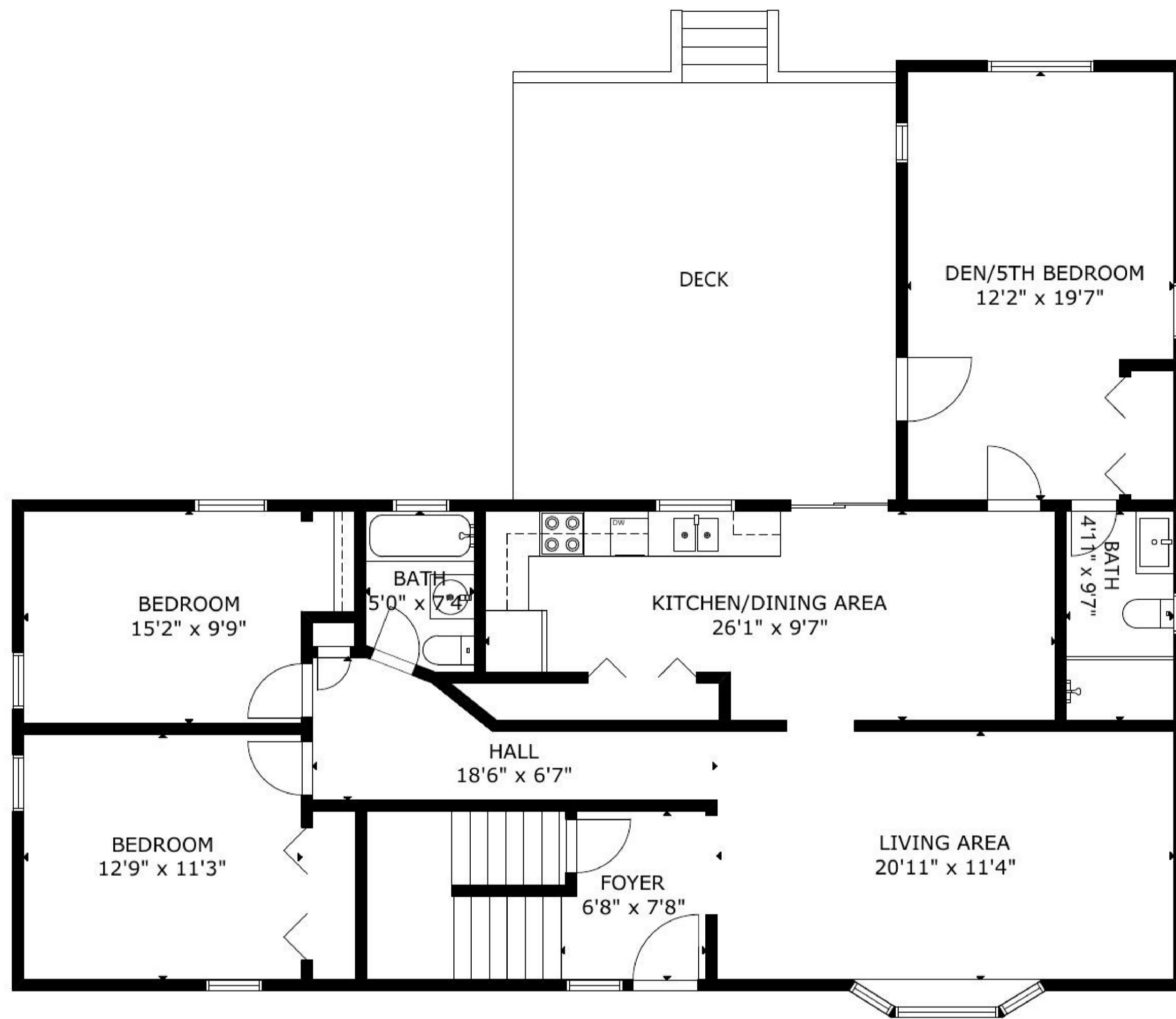
FIRST FLOOR
