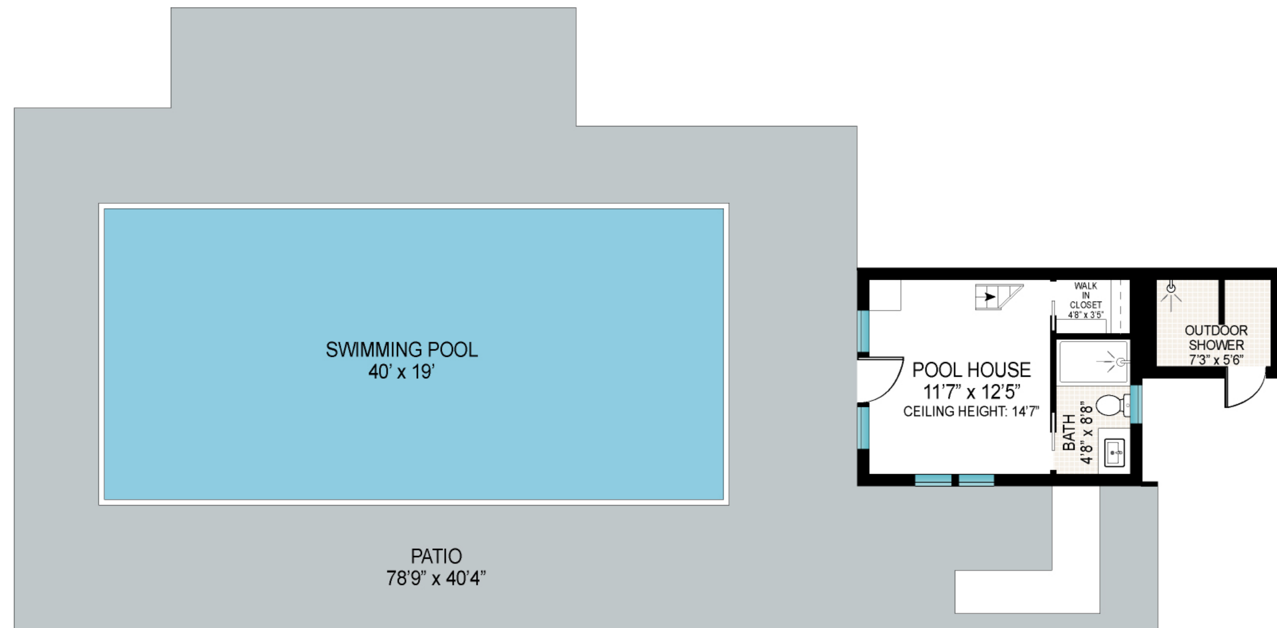
POOL HOUSE FIRST FLOOR
