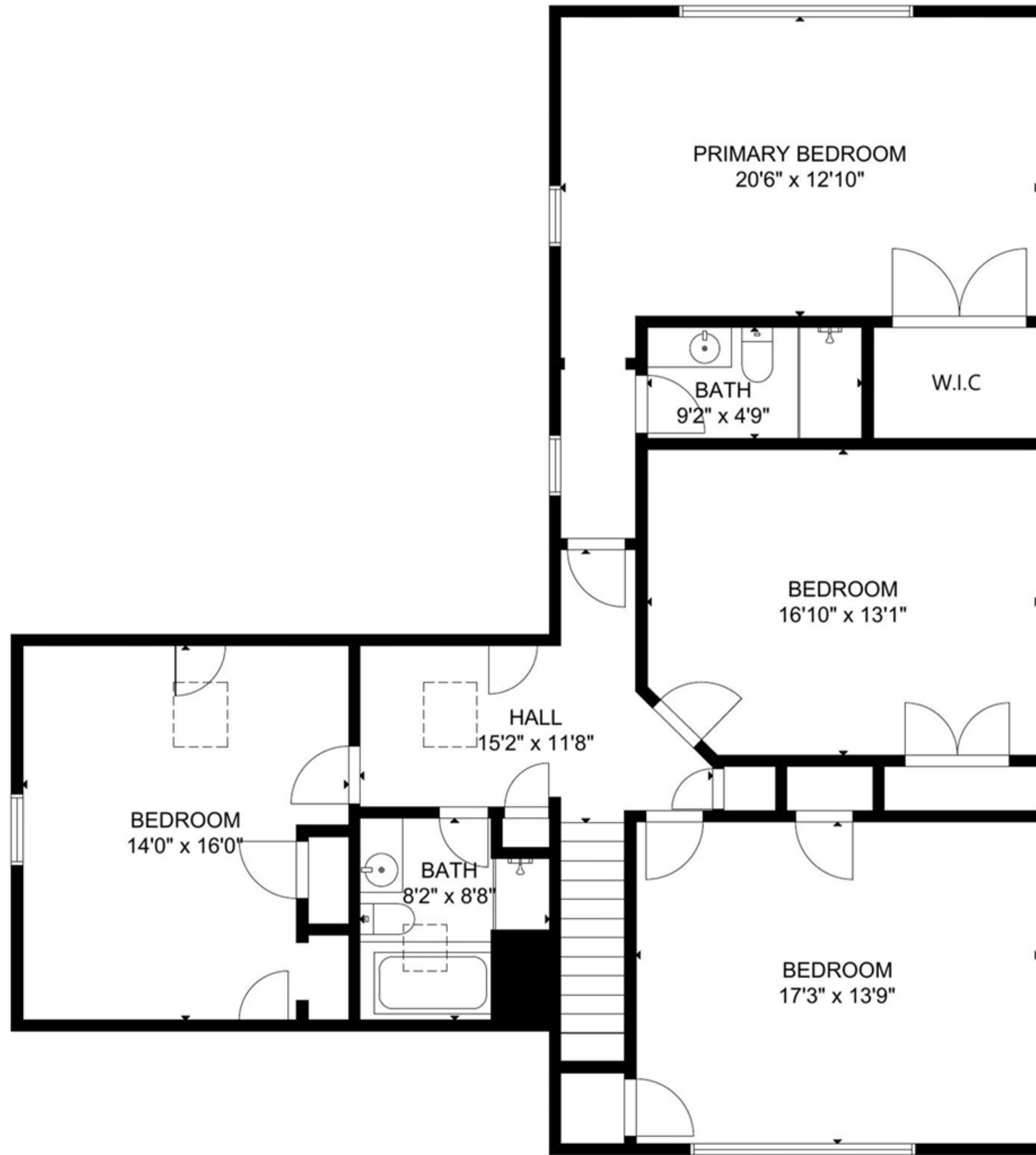
SECOND FLOOR
