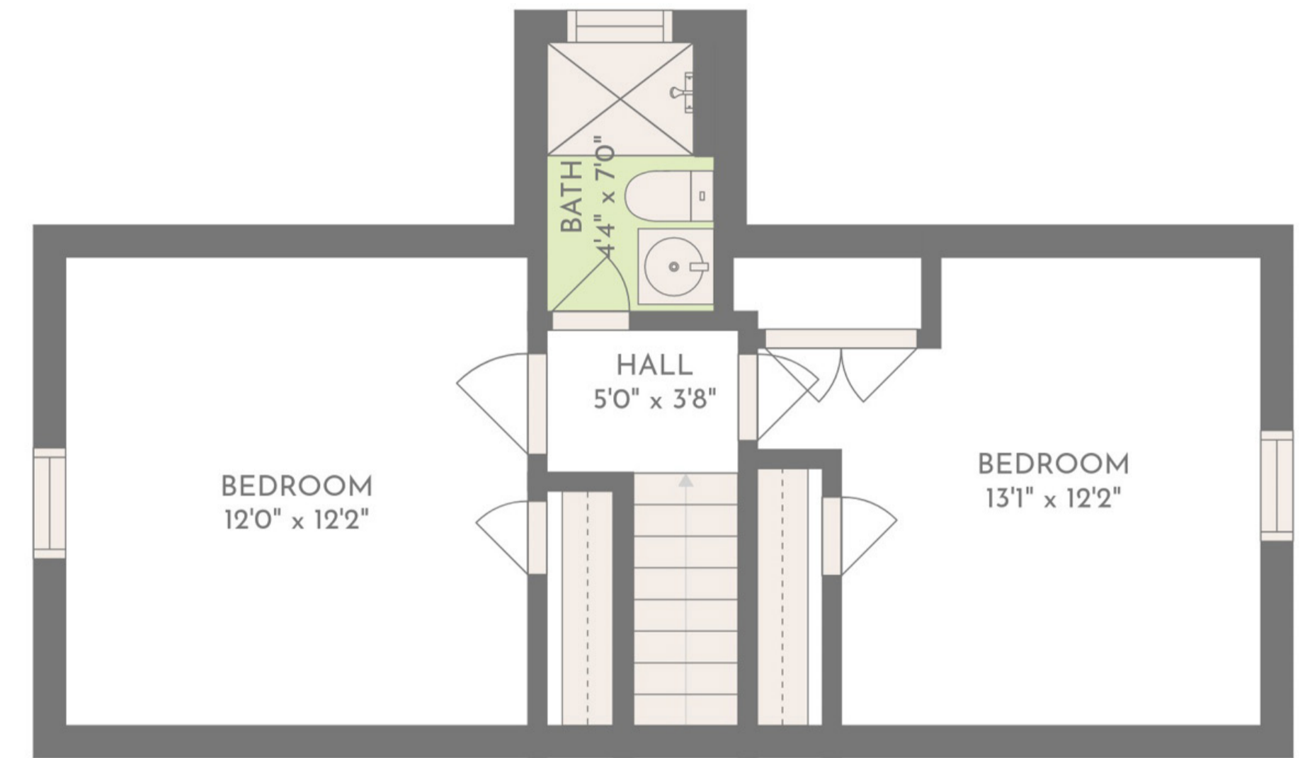
SECOND FLOOR
