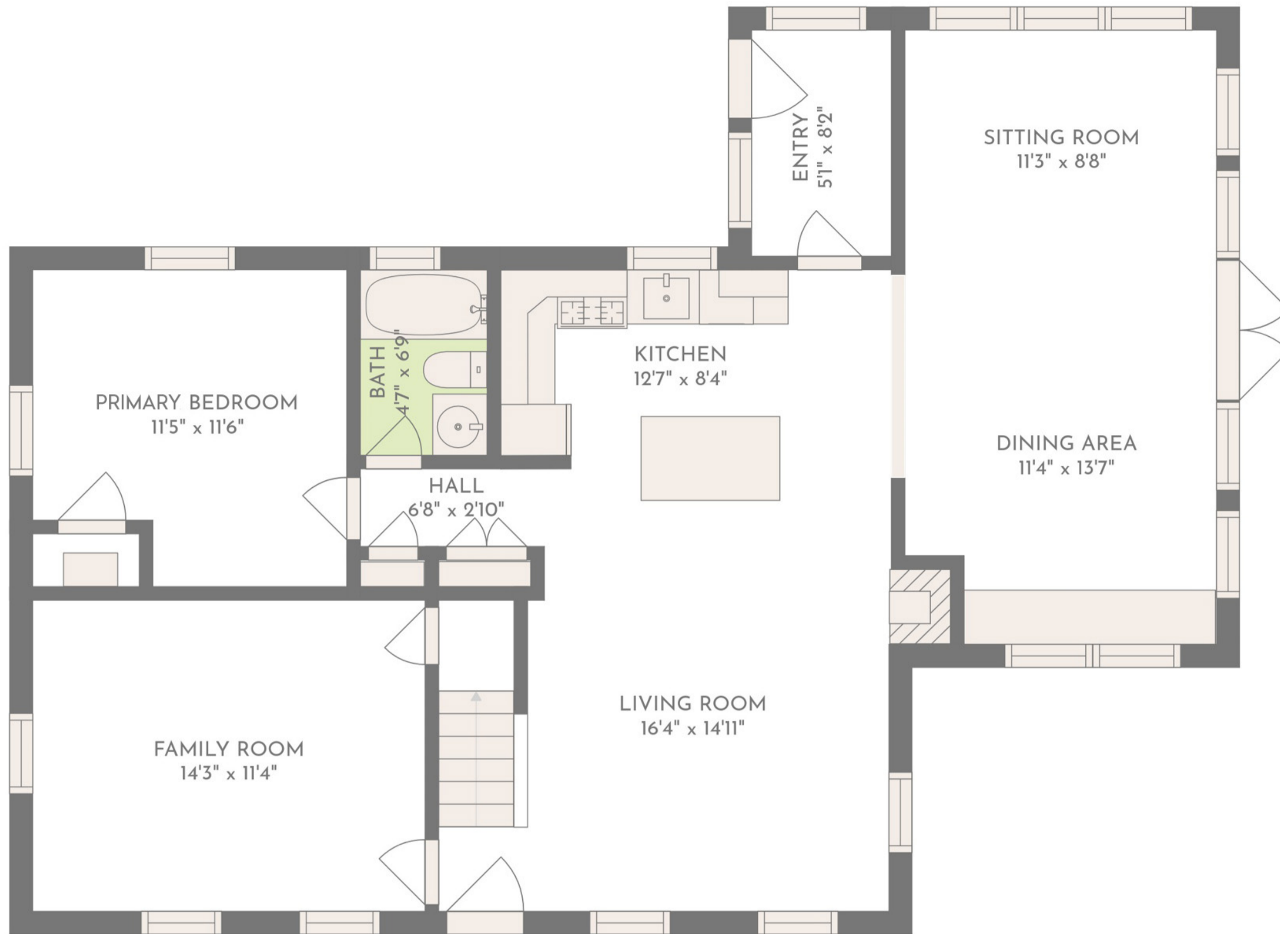
FIRST FLOOR
