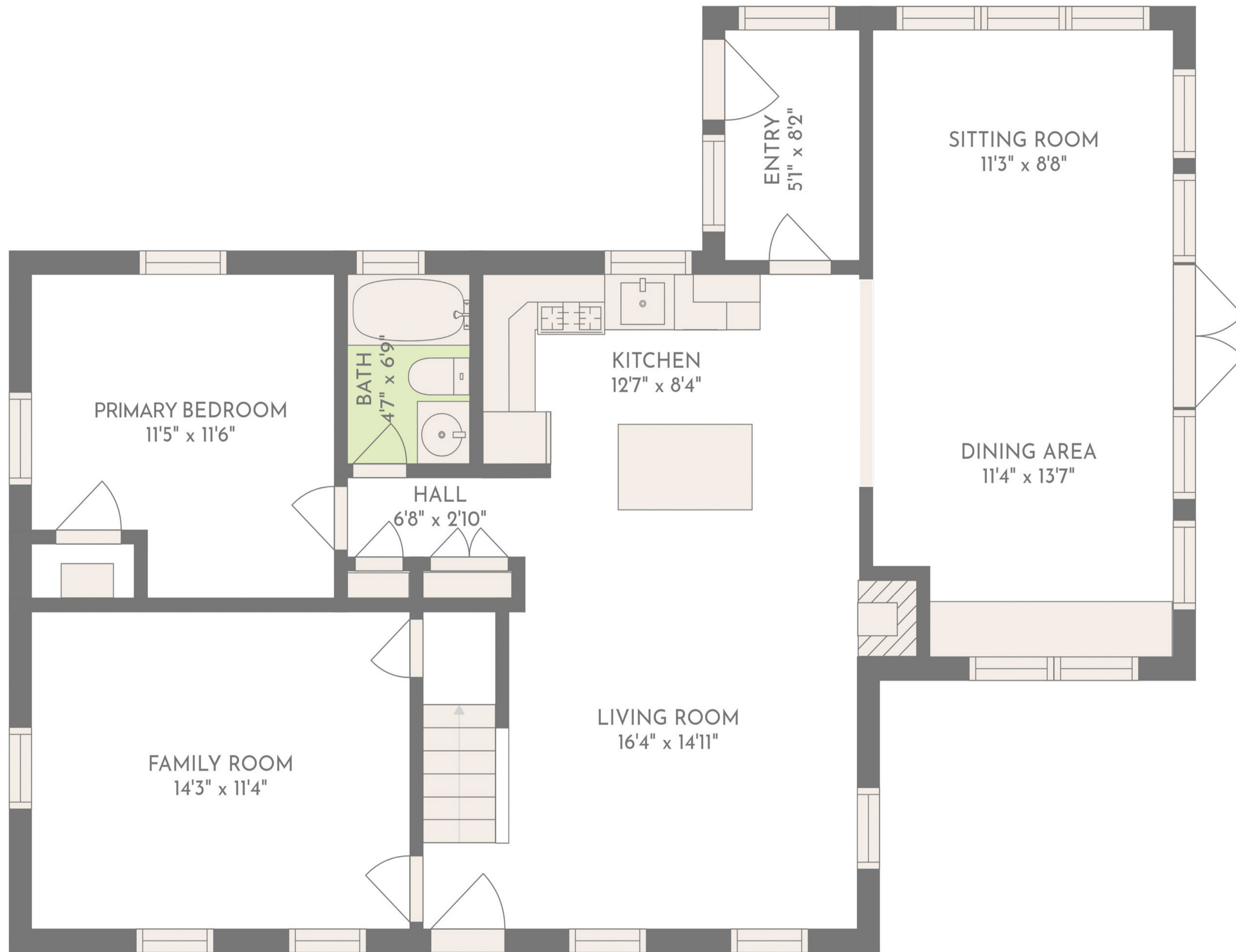
First Floor
