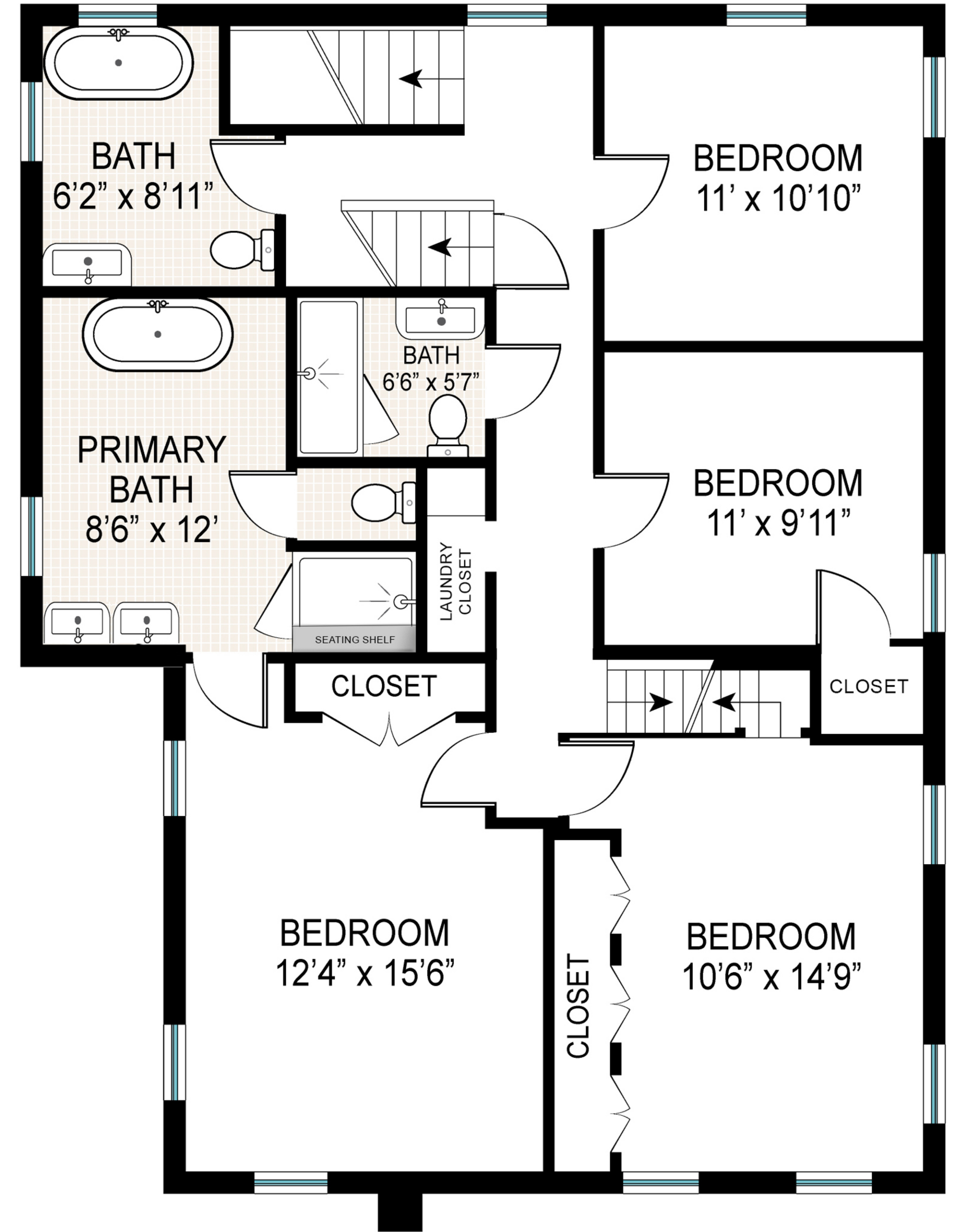
SECOND FLOOR
