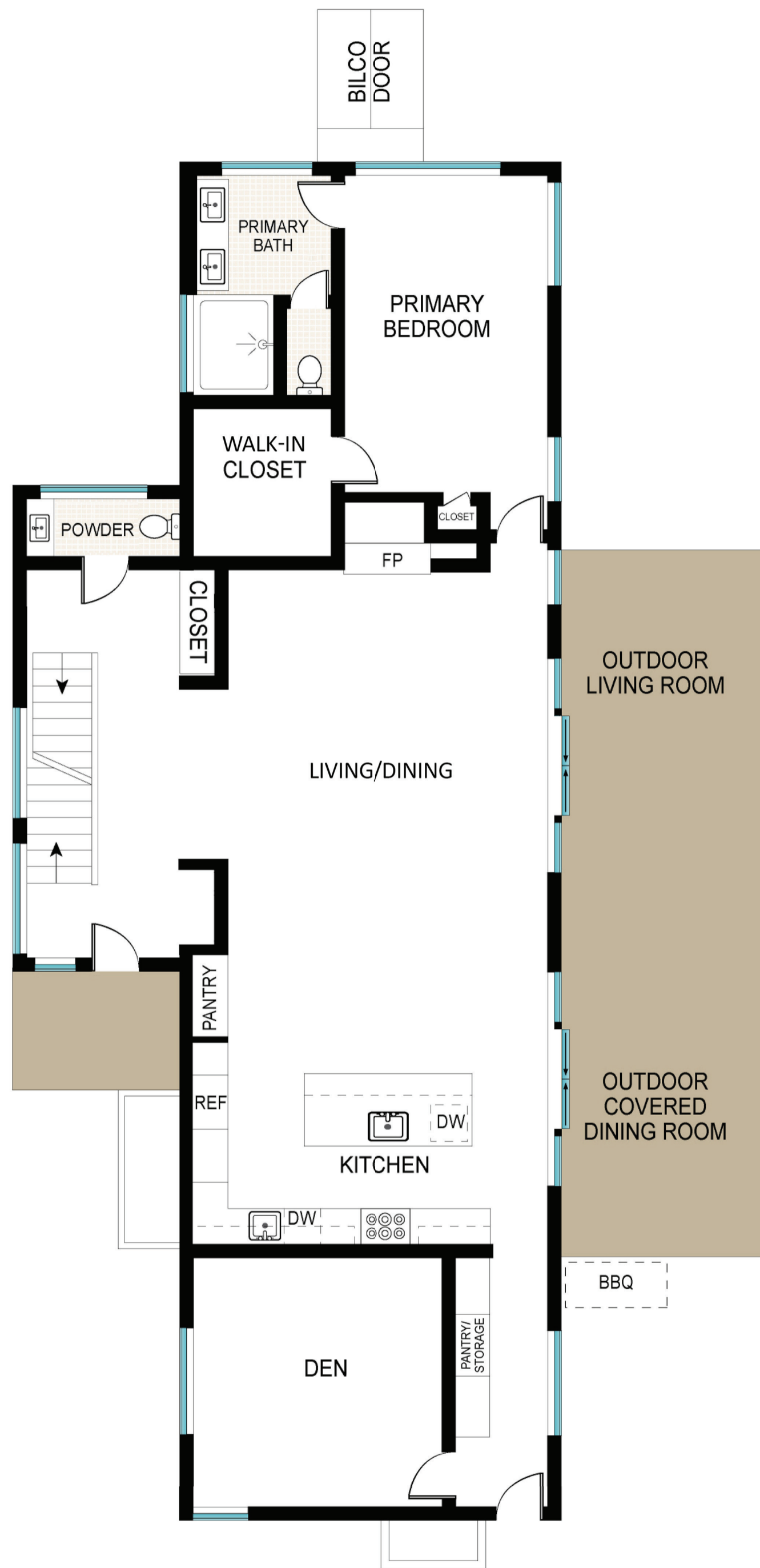
Ground Floor
