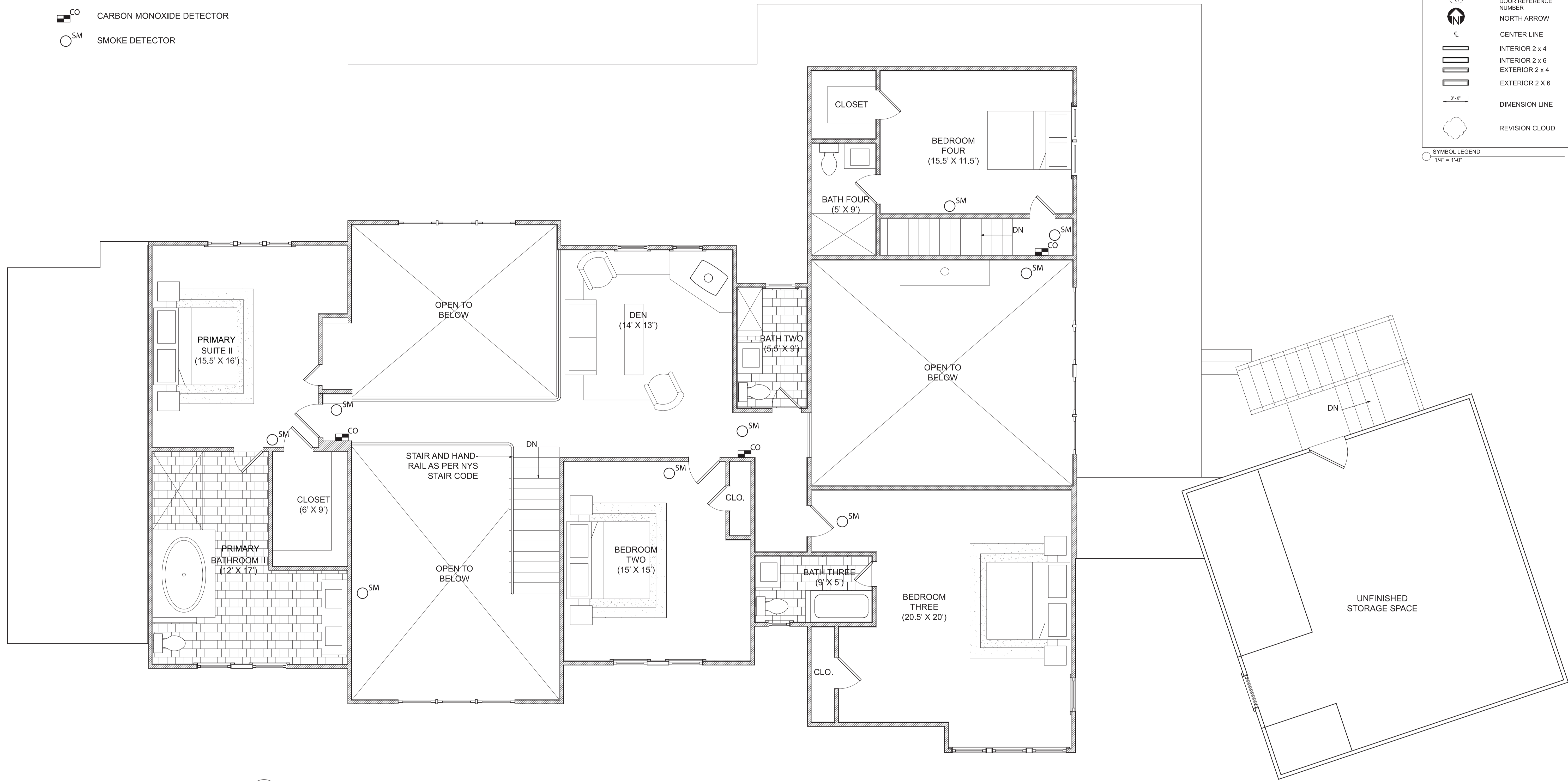
1 UPPER FLOOR PLAN 1/4" = 1'-0"
